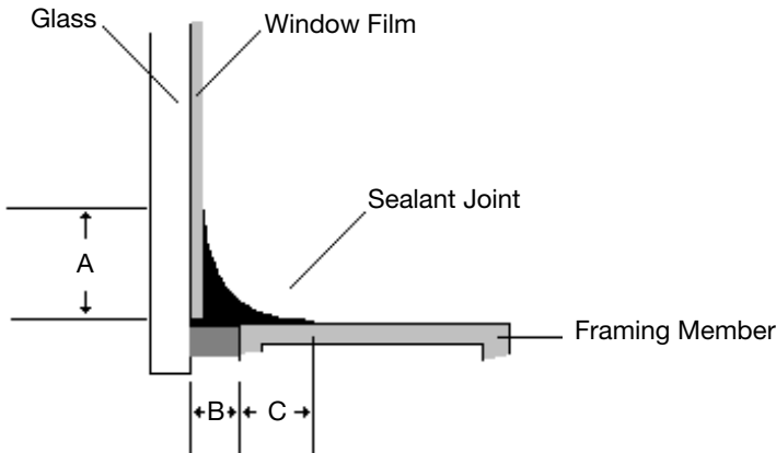
Figure 4. Concave joint surface (Unacceptable)
